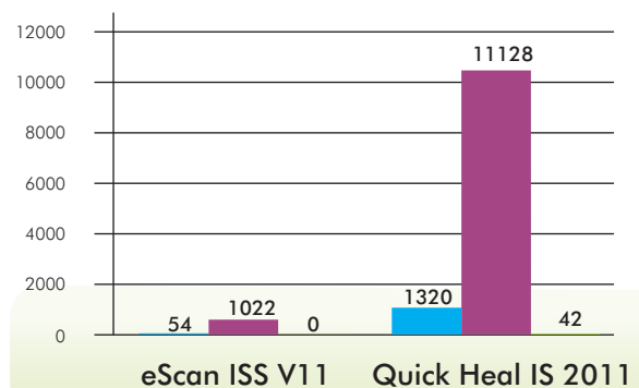
Source: VB100 (December 2010)
